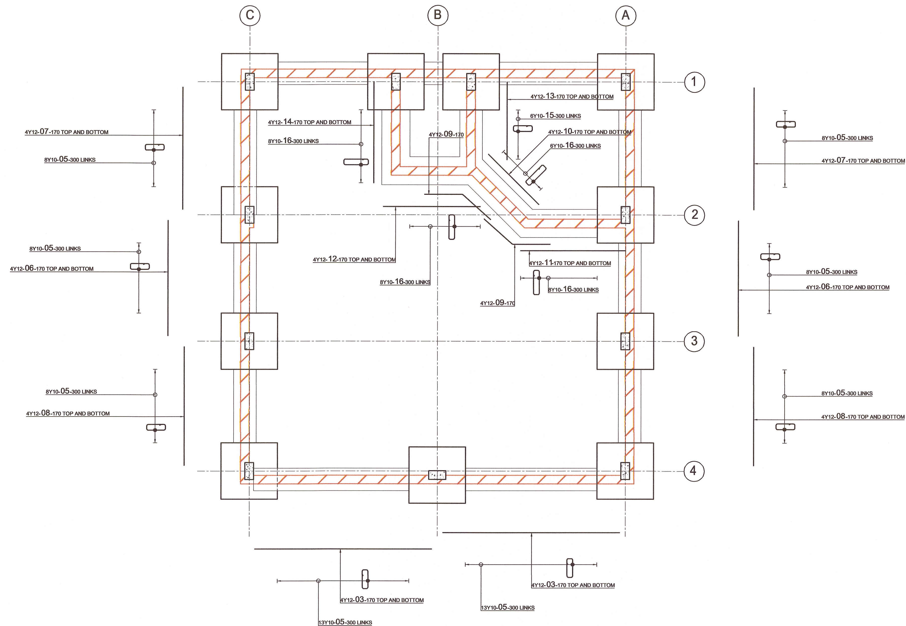
FOUNDATION LAYOUT
