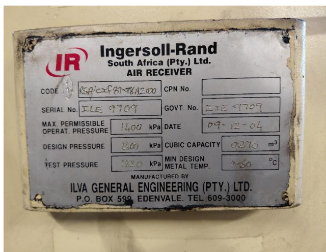
Picture 1: Compressor name plate.
