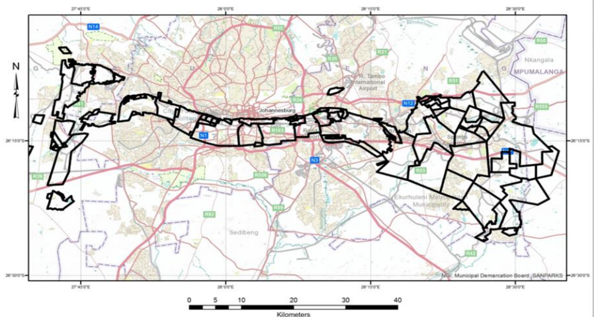
Figure 1. The Eastern, Central and Western, Basins of the Witwatersrand Goldfields
