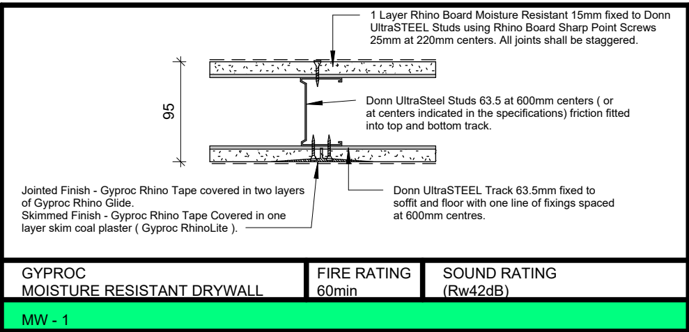
Drywall Detail 1 Scale: 1:5
