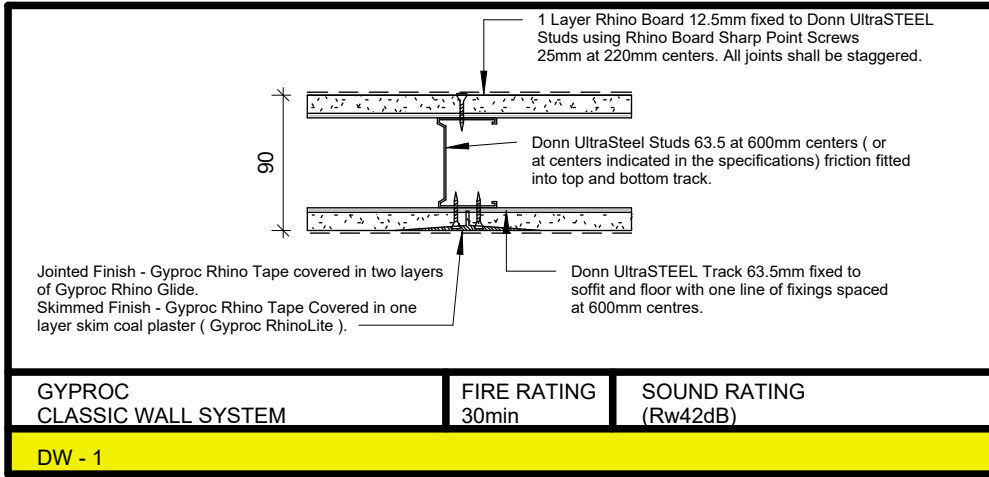
Drywall Detail 2 Scale: 1:5
