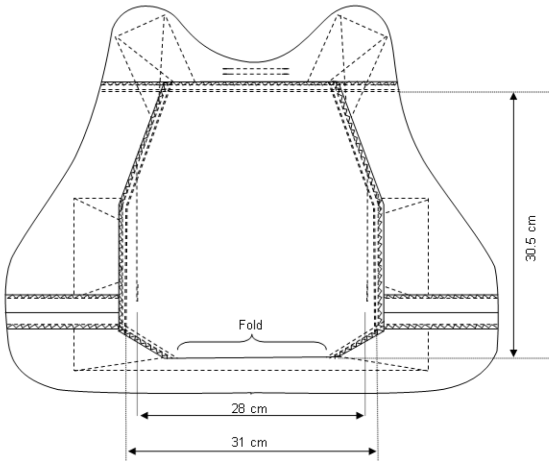
Figure 18 – Inside view of front outer panel
