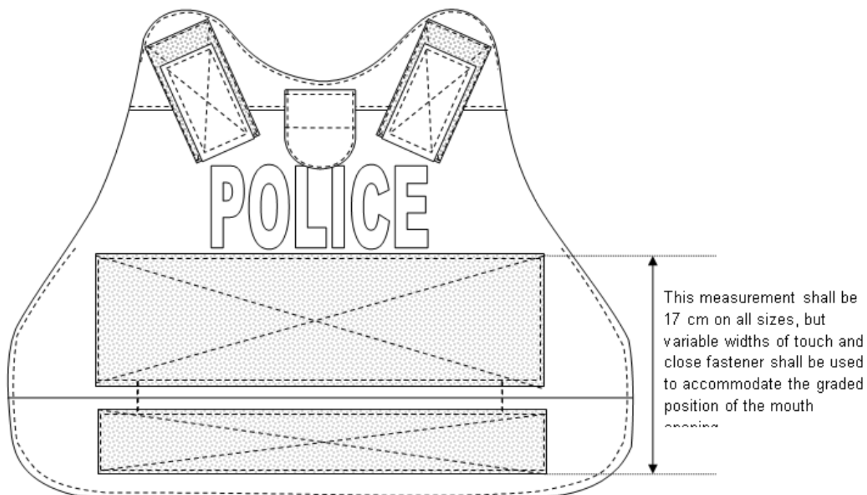
Figure 13(a) – Positioning of touch and close fastener
