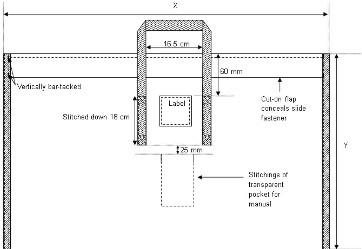
Figure 37 – Carry bag (see table 20)
