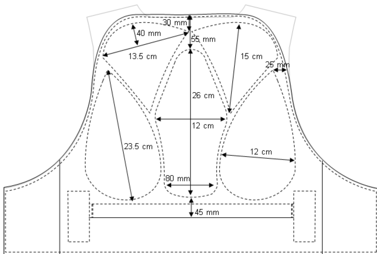
Figure 33 – Positioning and dimensions of the PATTERNS of the foam inserts in the lining of the back outer panel on a size MEDIUM which shall be graded on the other sizes
