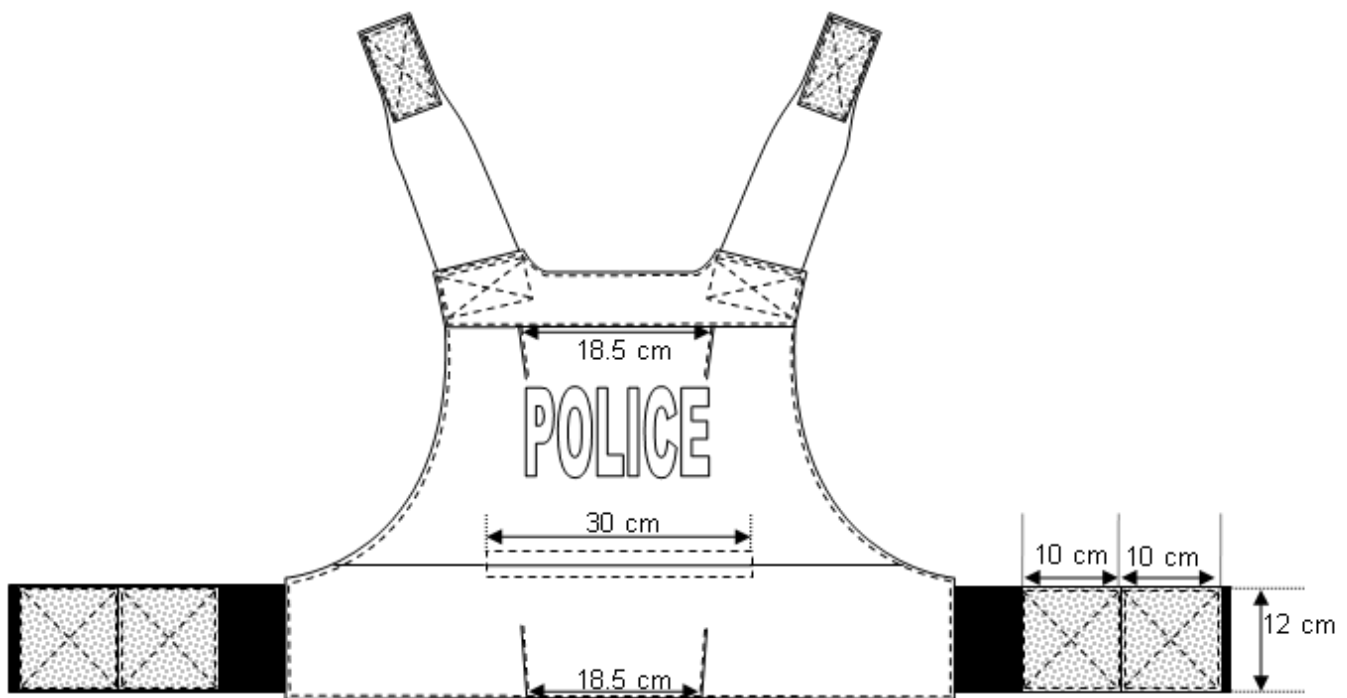
Figure 25 – Finished dimensions of design features on back outer panel
