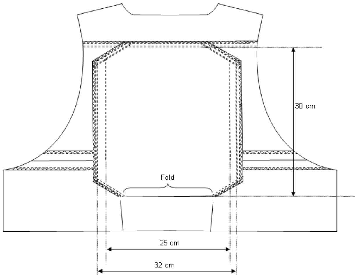
Figure 28 – Inside view of back outer panel
