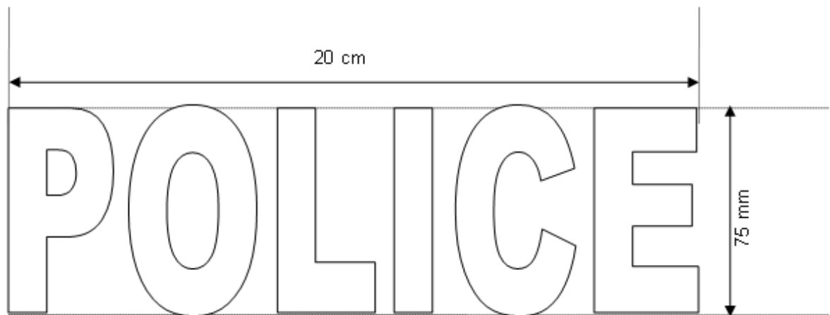
Figure 14 – Dimensions of printing on front and back outer panels
