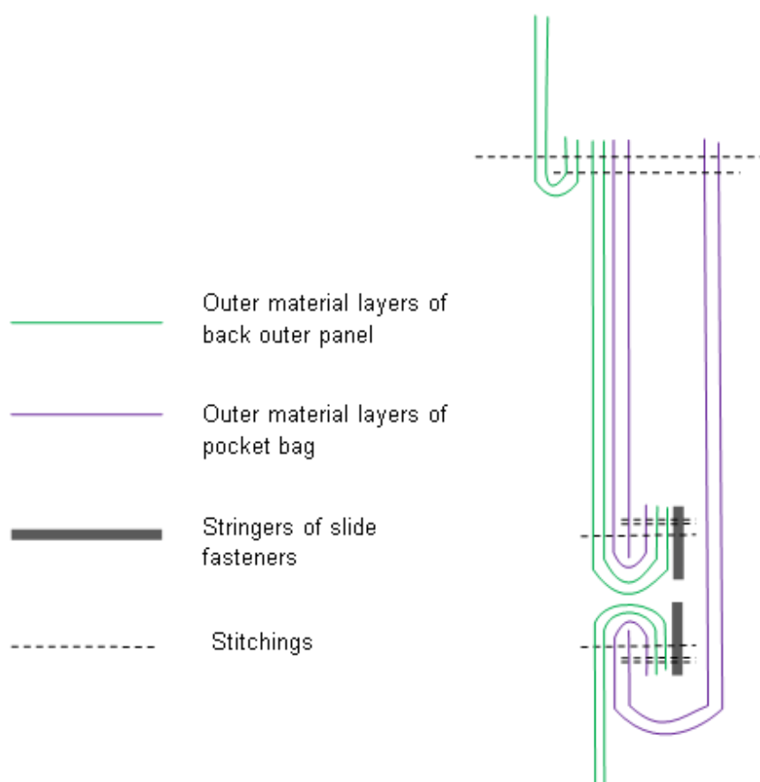
Figure 27 – Cross section of mouth opening on face side of back outer panel
