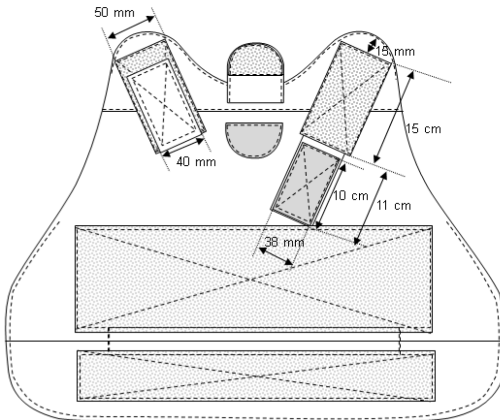
Figure 14 – Dimensions of printing on front and back outer panels
