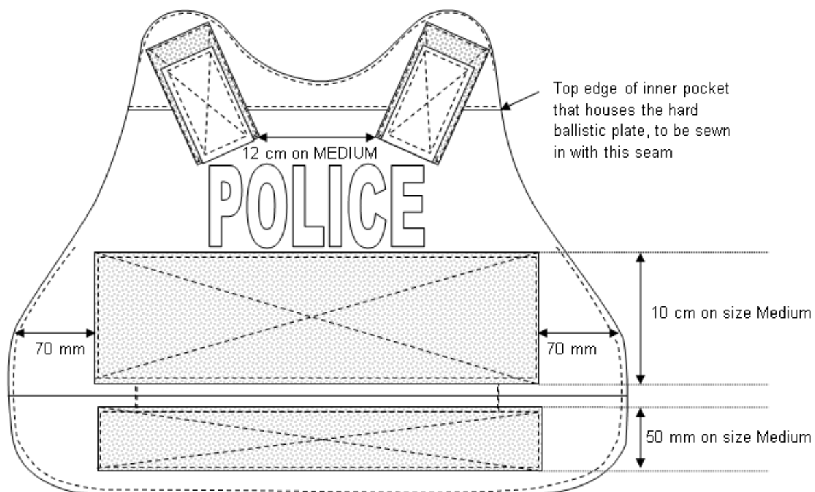
Figure 13(a) – Positioning of touch and close fastener
