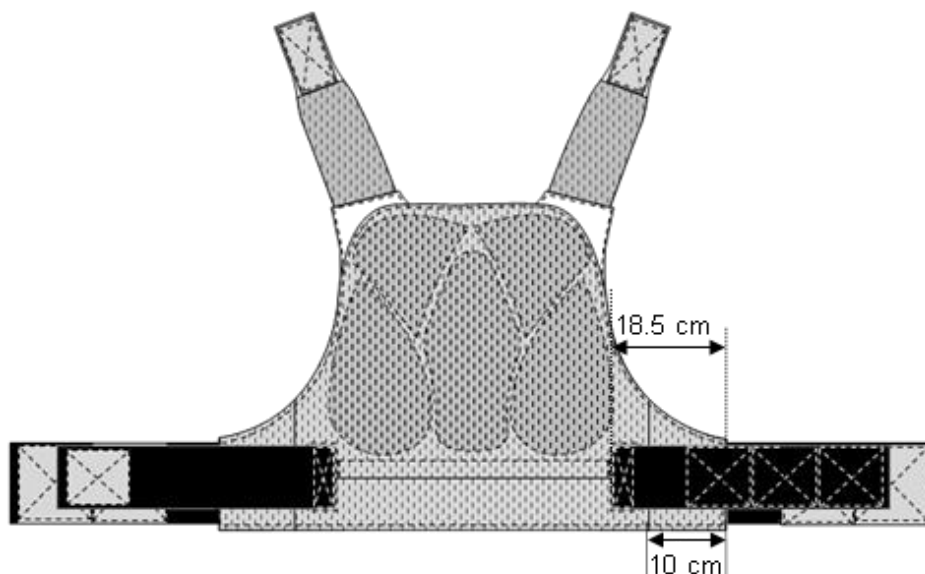
Figure 34 – Finished width of side section
