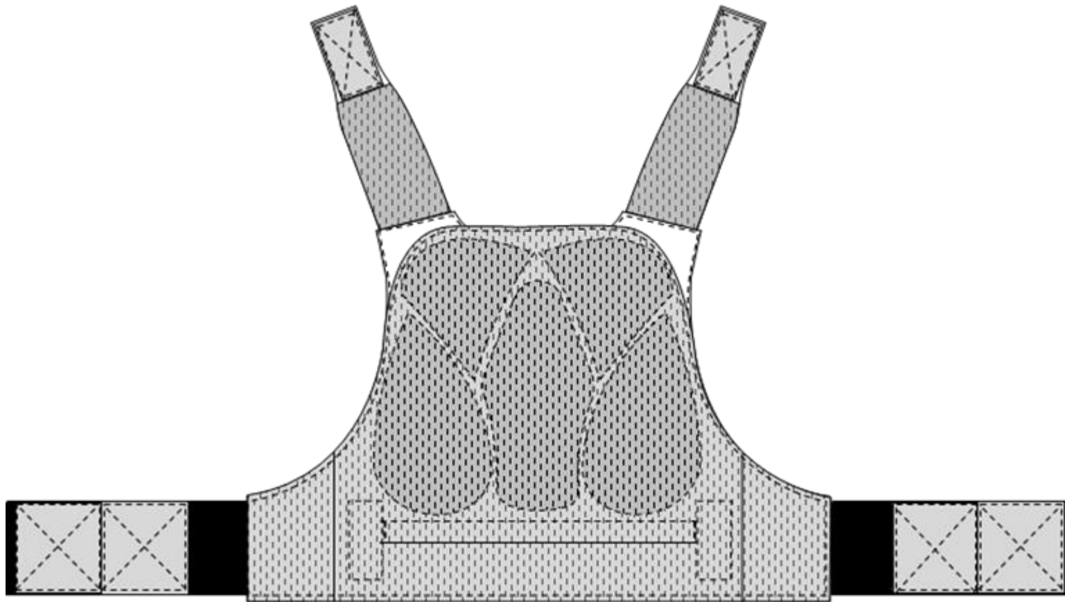
Figure 8(a) – Lining of back outer panel (inner waist support straps omitted in this illustration)
