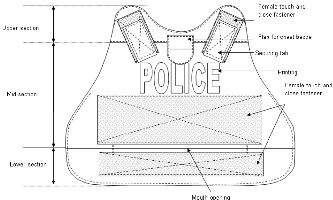
Figure 10 – Section identification and design features on face side of front outer panel
