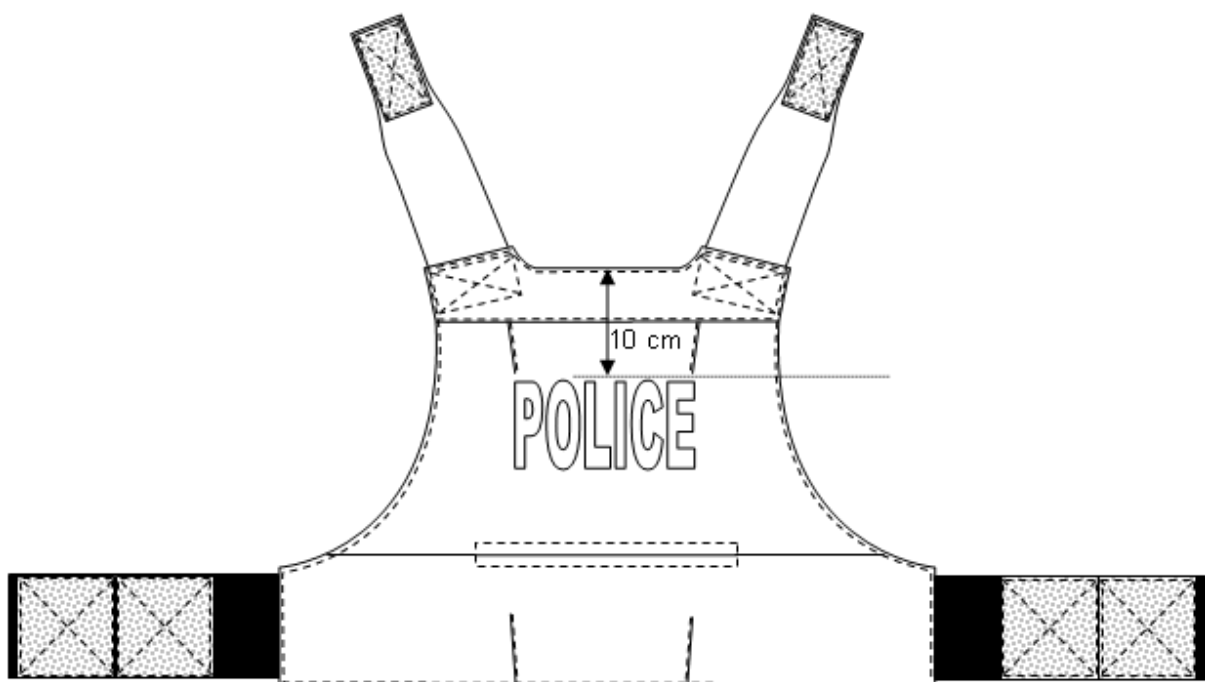
Figure 26 – Positioning of printing on the back outer panel
