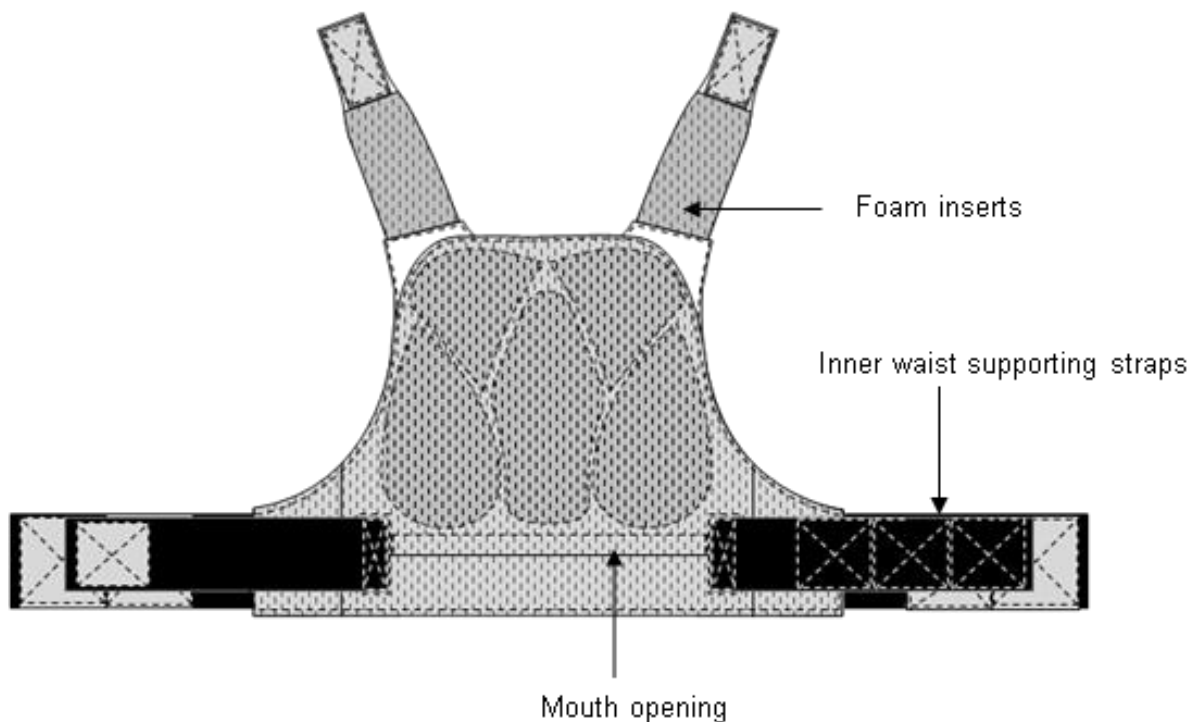
Figure 31 – Design features on lining of back outer panel
