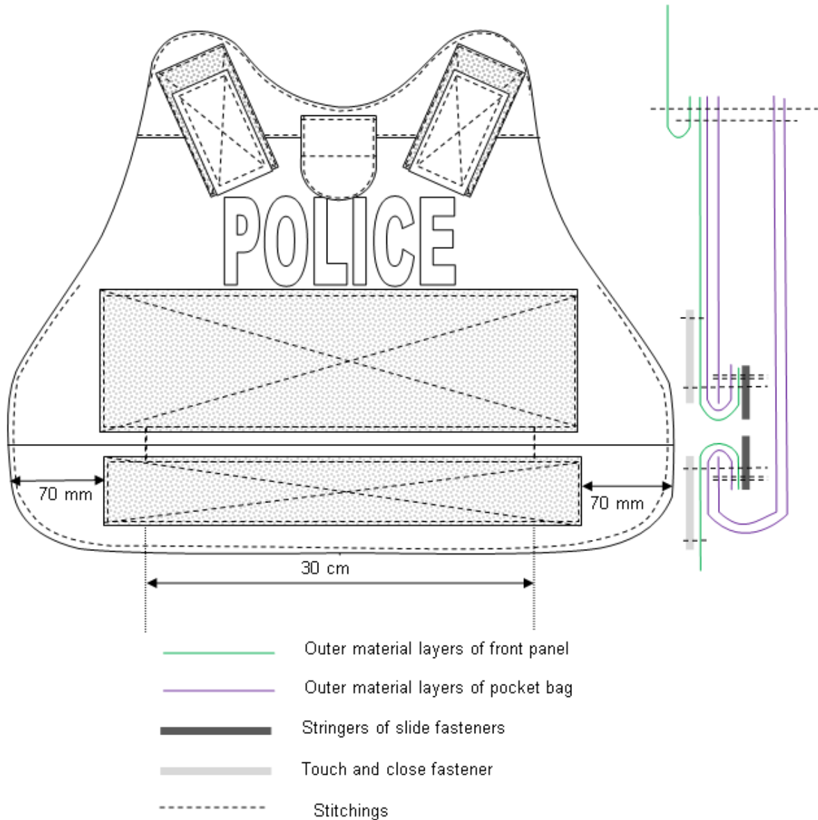
Figure 17 – Lower section dimensions and cross section of construction of front pocket
