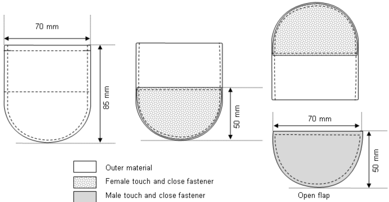
Figure 11 – Flap for attachment of embossed chest badge
