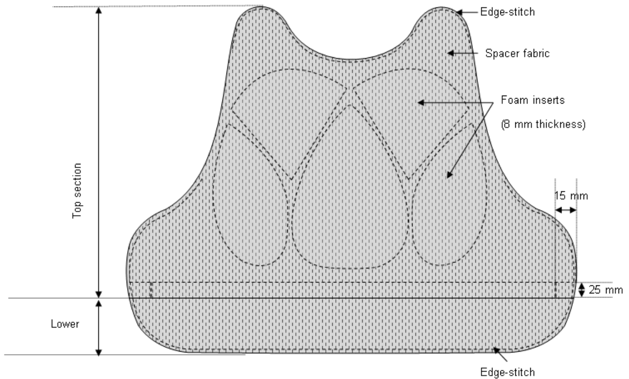
Figure 19 – Lining of front outer panel
