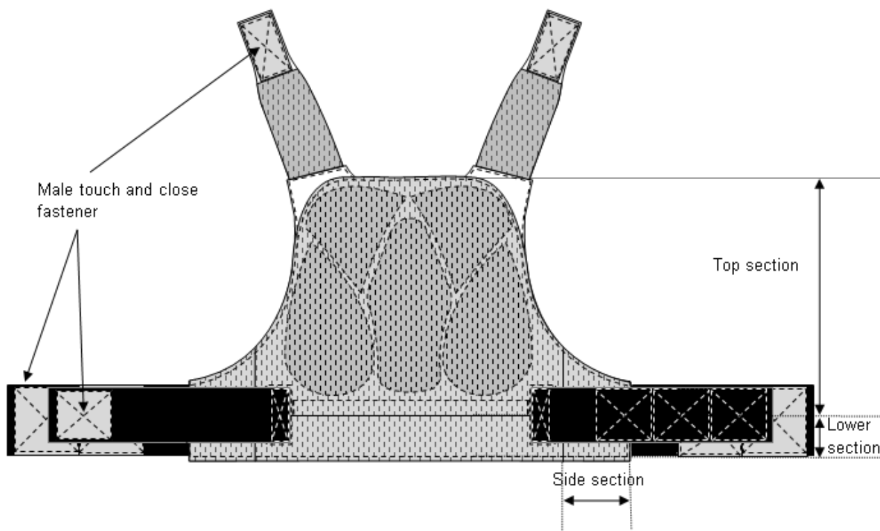
Figure 30 – Identification of sections of lining of the back outer panel
