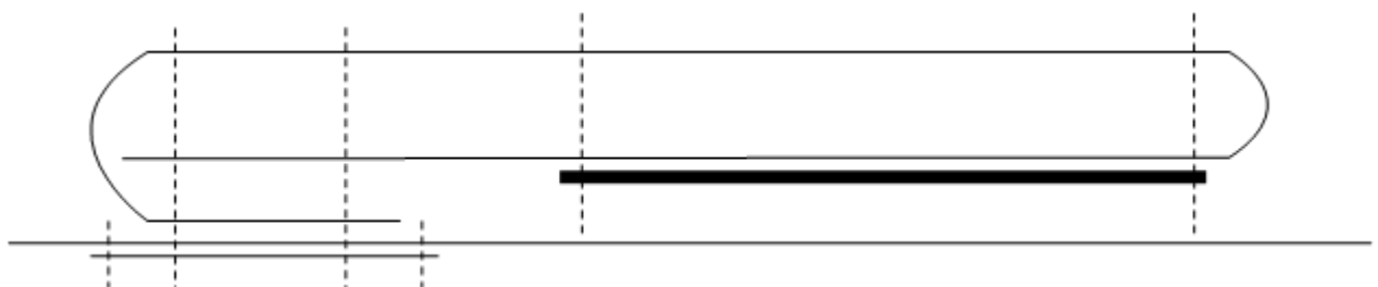
Figure 35(a) – Cross section of construction of left inner waist support strap when 80 mm wide touch and close fastener is used (refers to as when worn)
