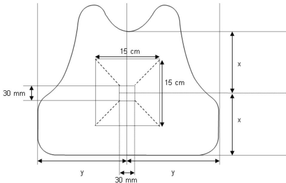
Figure 36 – Cross stitch on front soft ballistic armour pack
