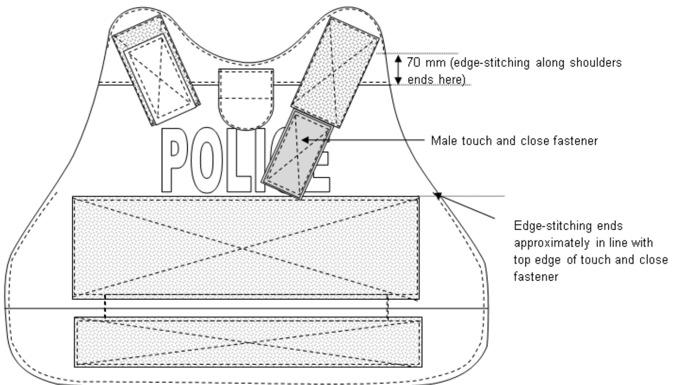
Figure 12 – Positioning of edge-stitchings around the outer edges of the front outer panel
