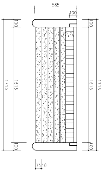
TOP VIEW SCALE 1:20
