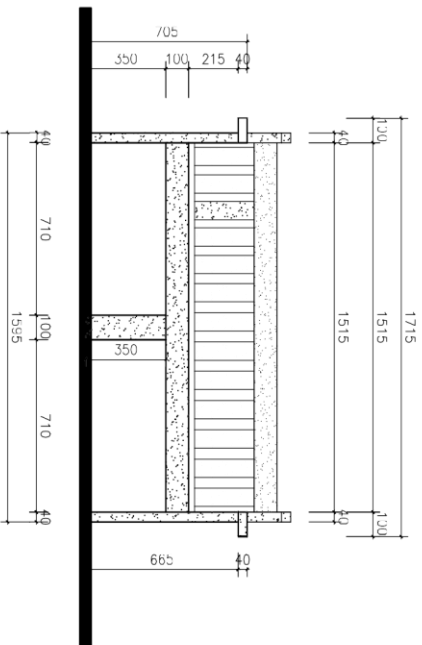
FRONT VIEW SCALE 1:20
