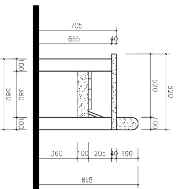
SIDE VIEW SCALE 1:20
