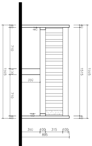
BACK VIEW SCALE 1:20
