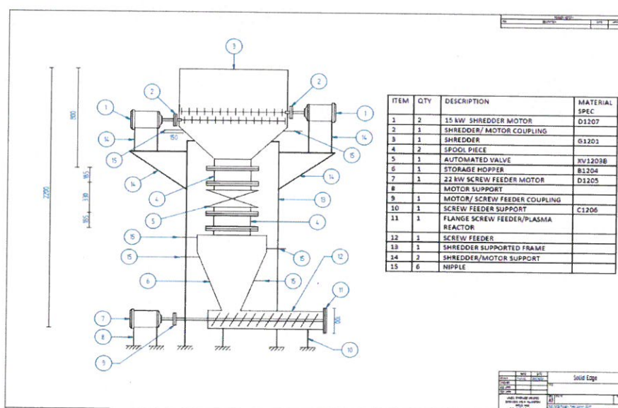
Figure 1 : Shredder, feed-hopper and screw-feeder 2D sketch
