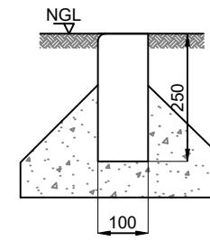
ROADWAY EDGING
