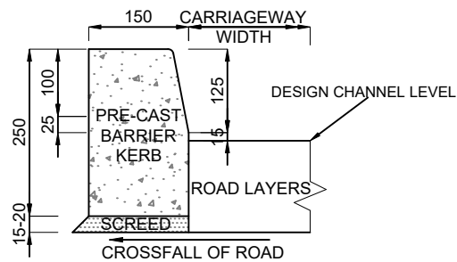
PRE-CAST BARRIER KERB WITH CAST-IN-SITU AND CHANNEL WITH 100mm BASE COURSE
