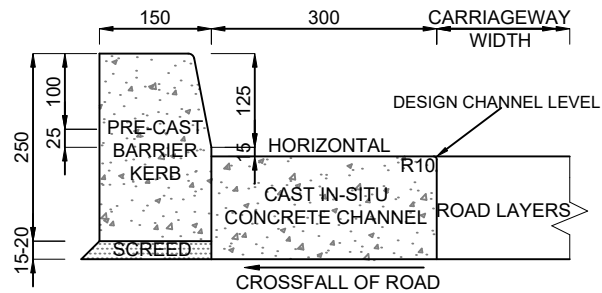
PRE-CAST BARRIER KERB WITH CAST-IN-SITU AND CHANNEL WITH 100mm BASE COURSE
