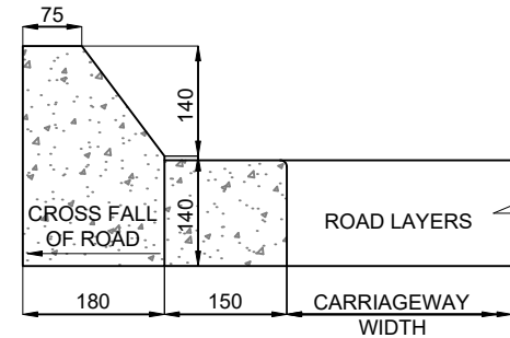
FIG 7 MOUNTABLE KERB AND CHANNEL
