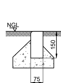
FOOTWAY EDGING
