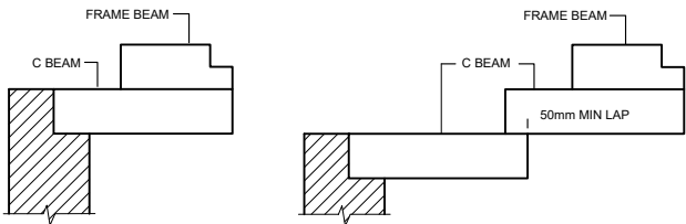
TYPICAL LAYOUTS FOR POSITIONING OF C BEAMS
