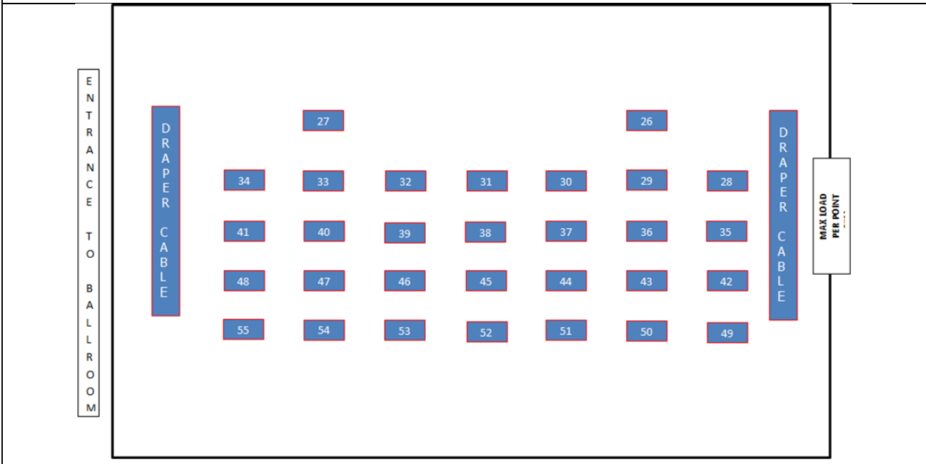
C2. Ballroom West Rigging Points Layout
