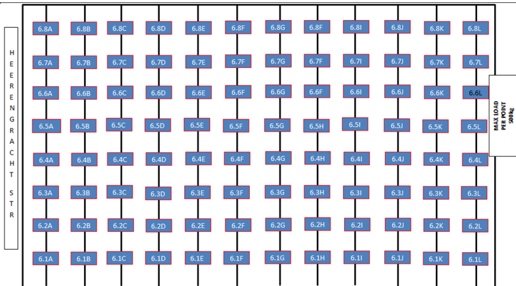
D4. Hall 7 Rigging Points Layout
