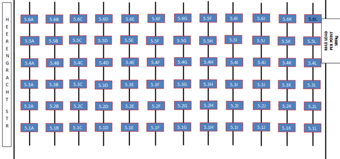
D6. Hall 9 Rigging Points Layout
