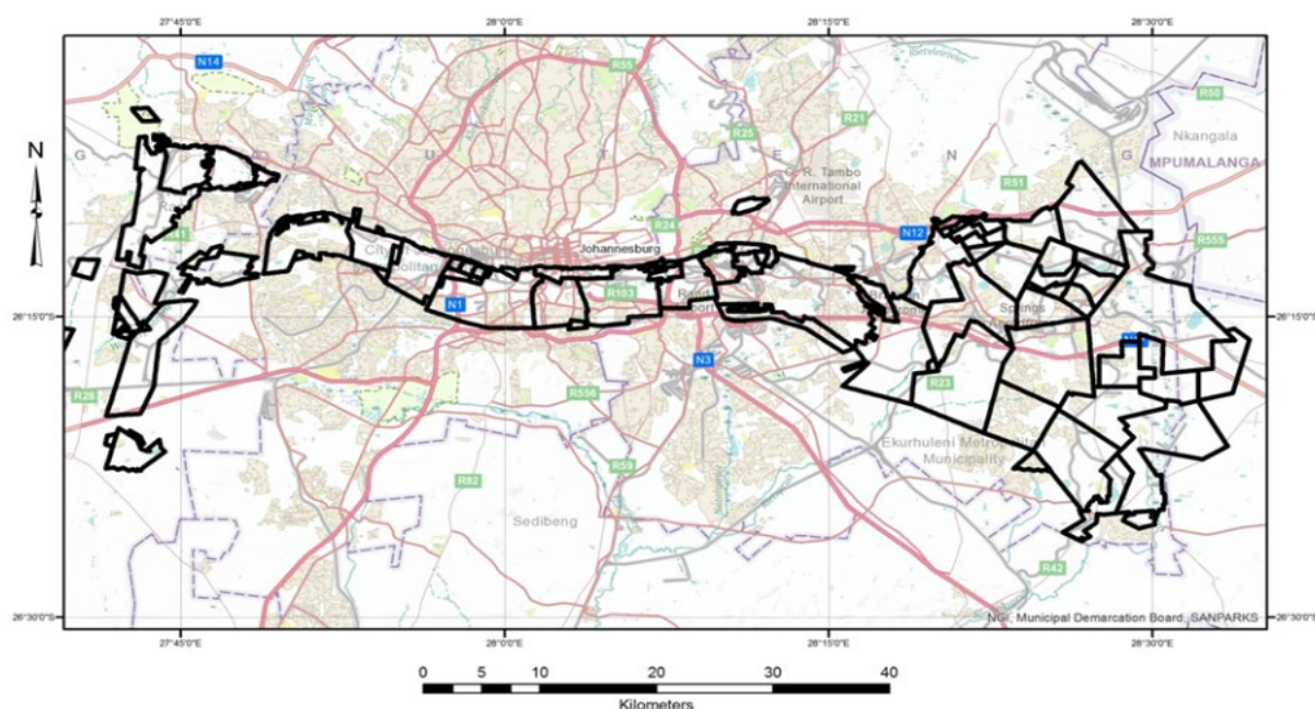
Figure 1. The Eastern, Central and Western, Basins of the Witwatersrand Goldfields
