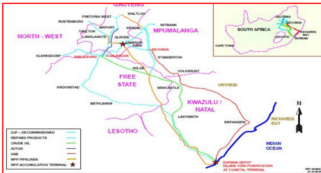
Figure 1: Transnet Pipeline Network
