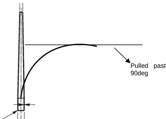
Figure 2: Bird perch diverter longitudinal pull test
