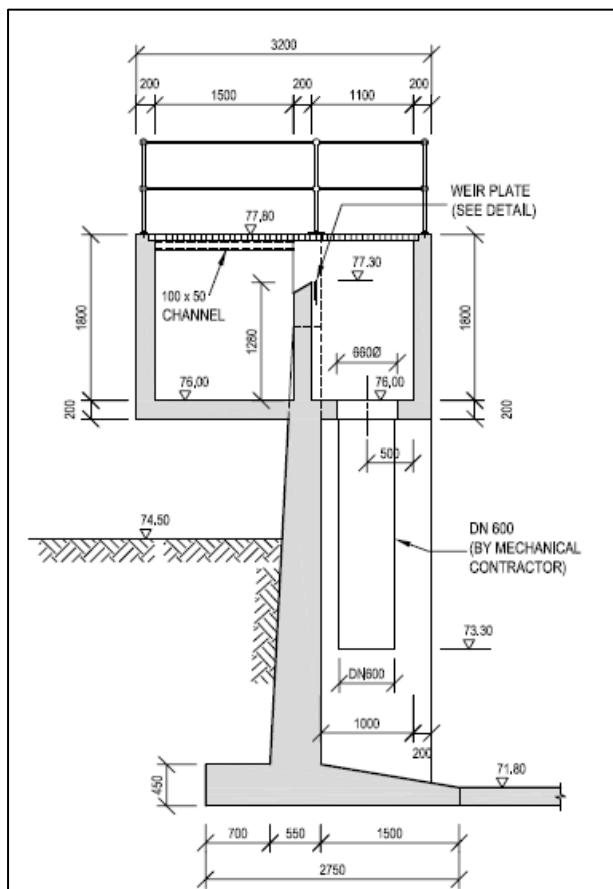
Fig 1:Sunderland Ridge WWTW general arrangement
