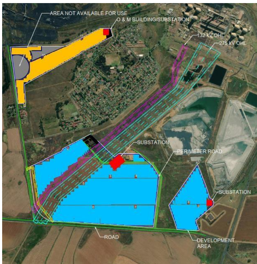
Figure 3: Indicative overall development areas for Solar PV
