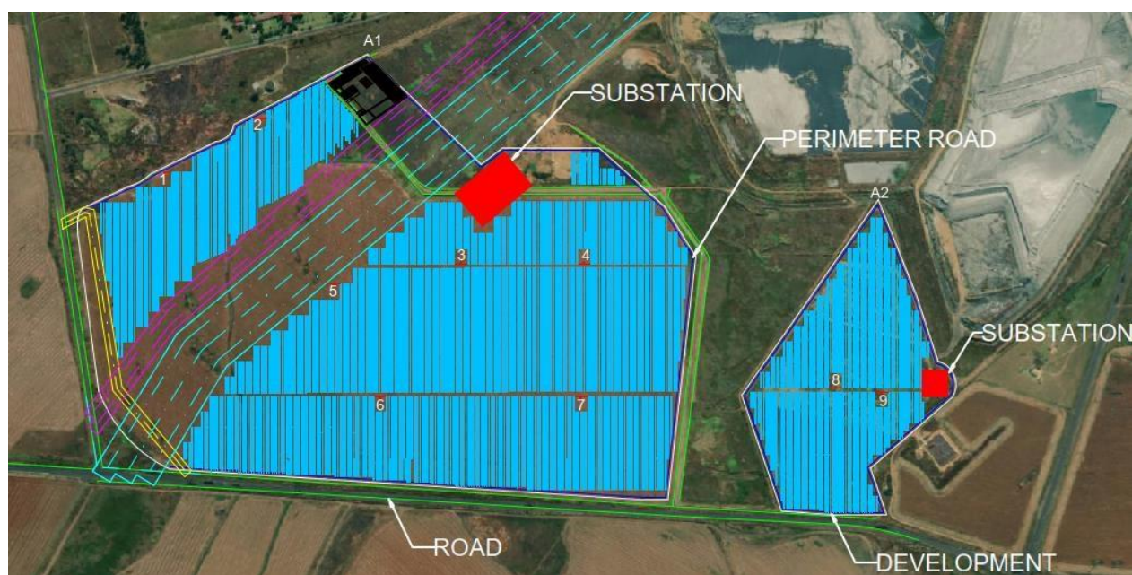
Figure 2: Indicative development area for Komati Solar PV Site A
