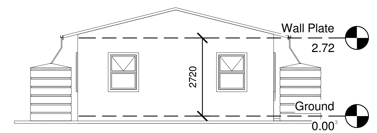
5 WEST ELEVATION 1 : 100
