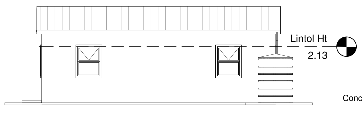
2 NORTH ELEVATION 1 : 100
