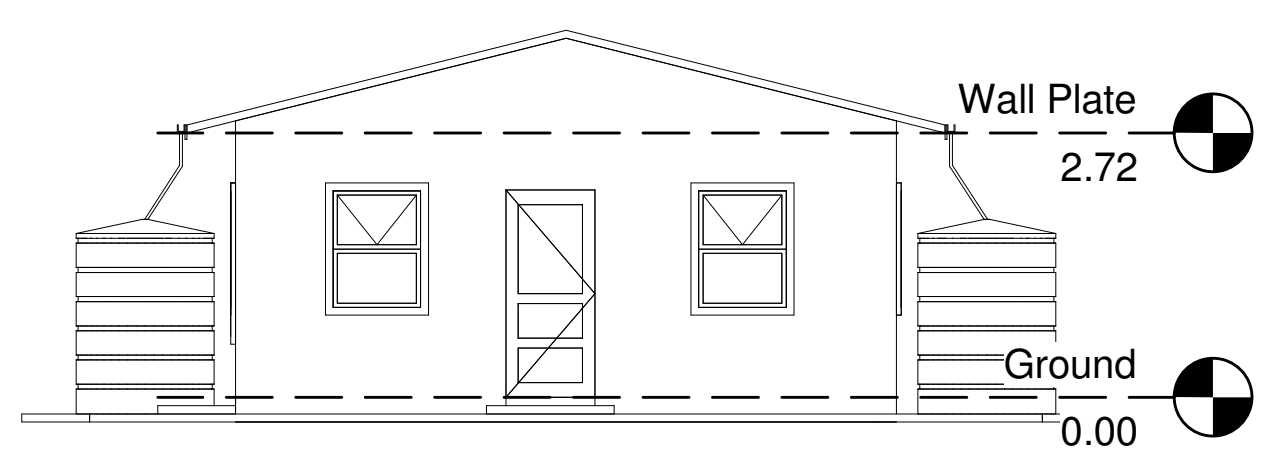
4 EAST ELEVATION 1 : 100
