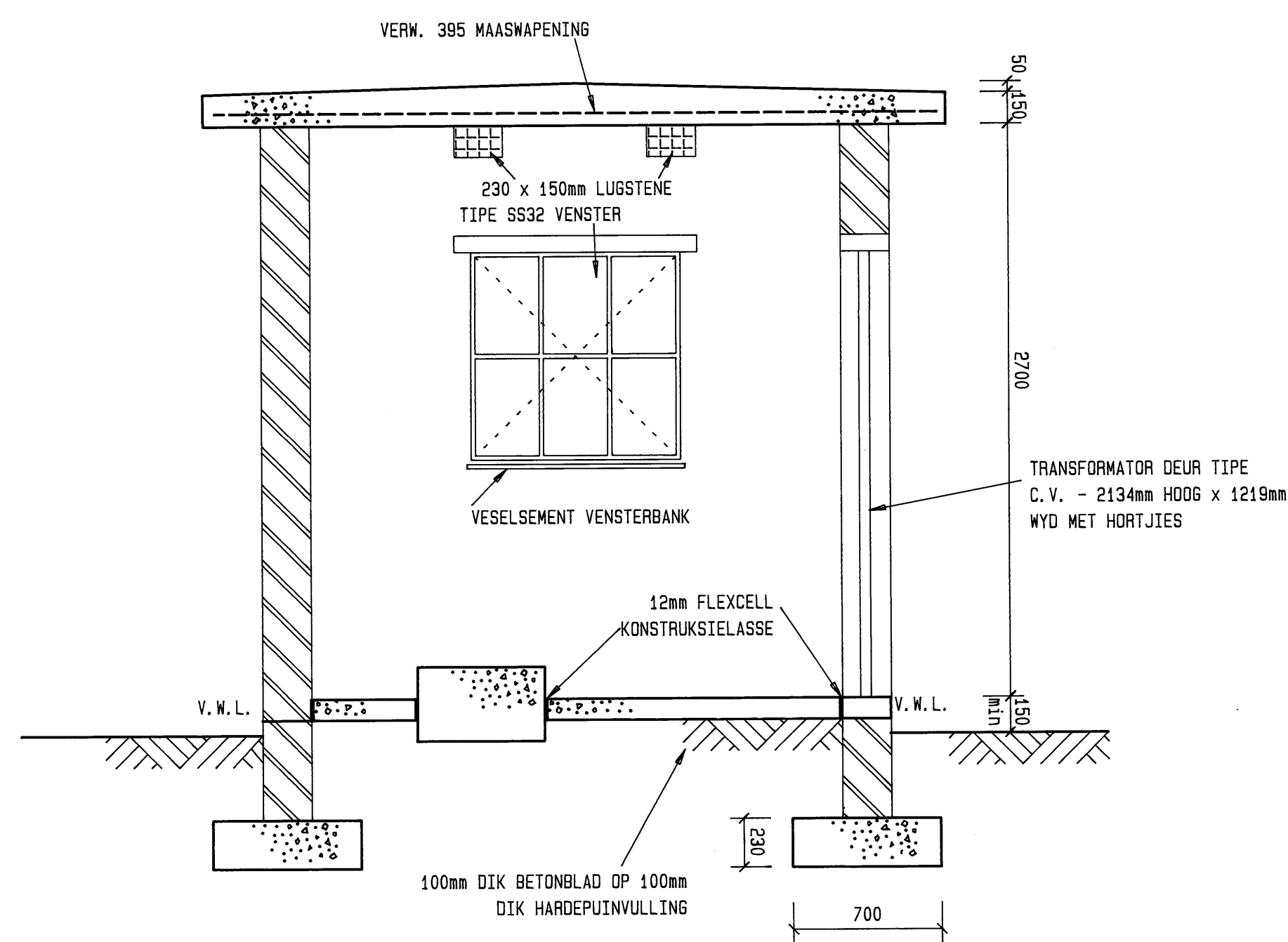
SNIT A - A
