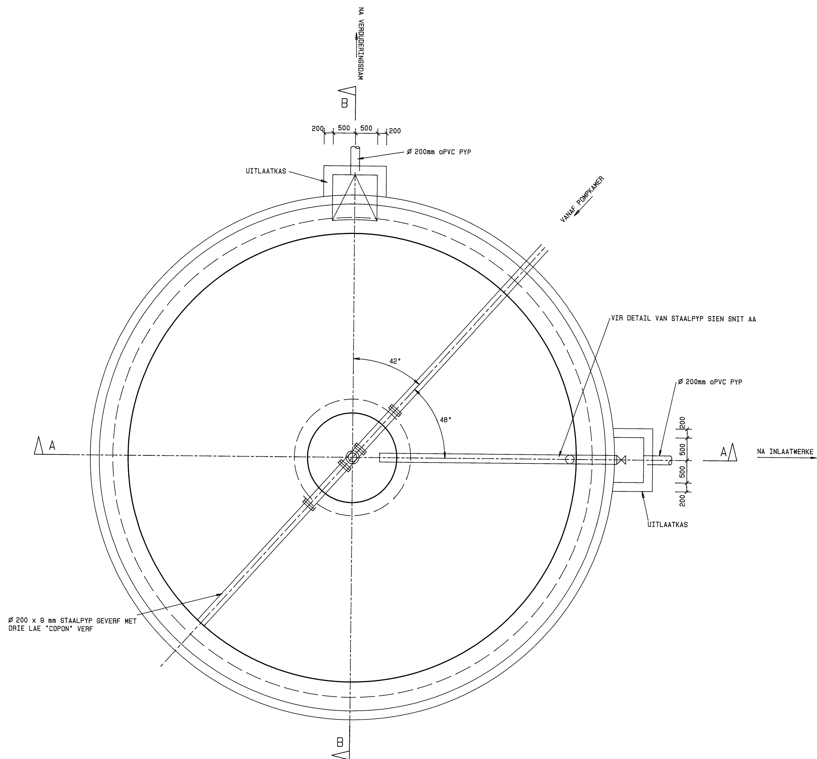
PLAN
