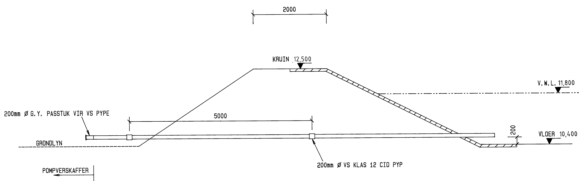
SNIT E - E: SUIGPYP BY LEIDAM 1 : 50
