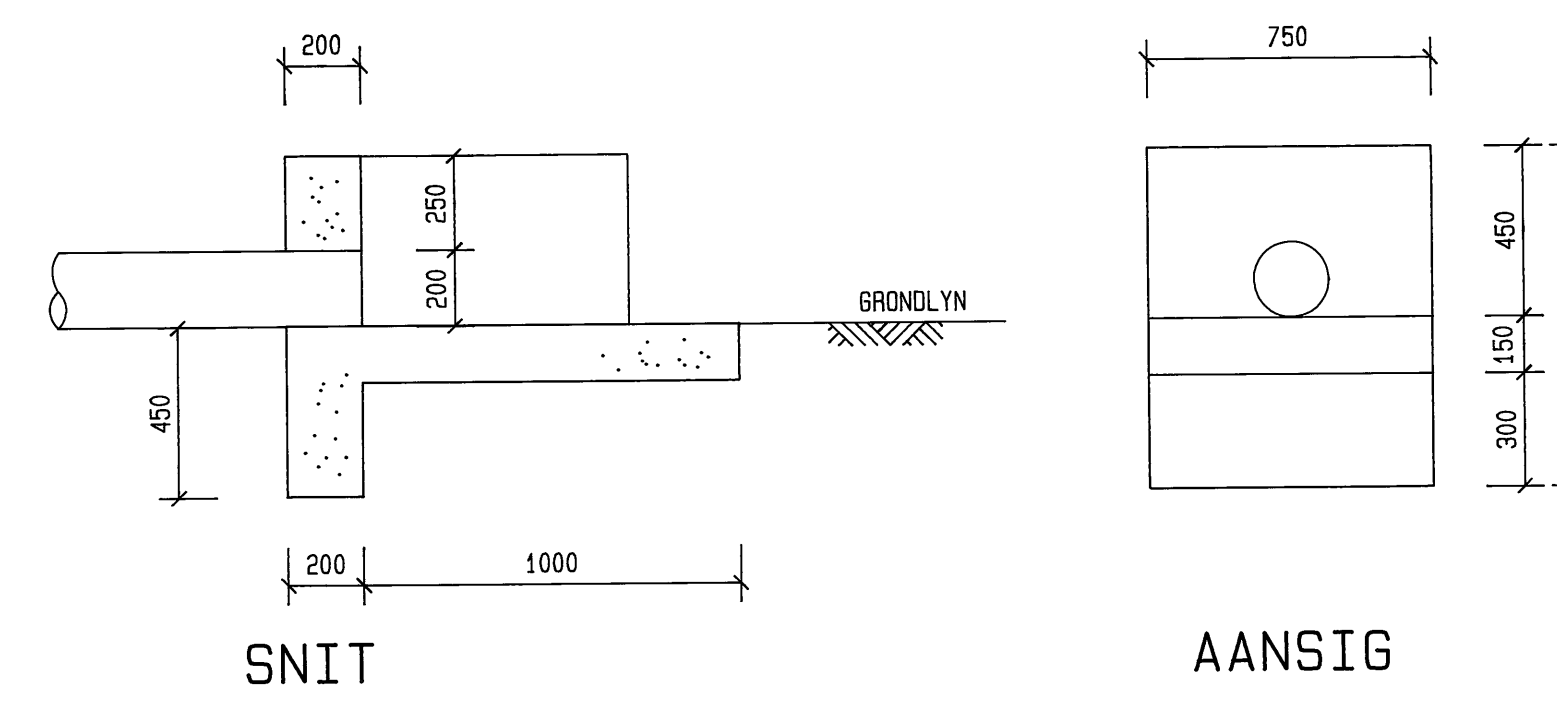
SNIT
