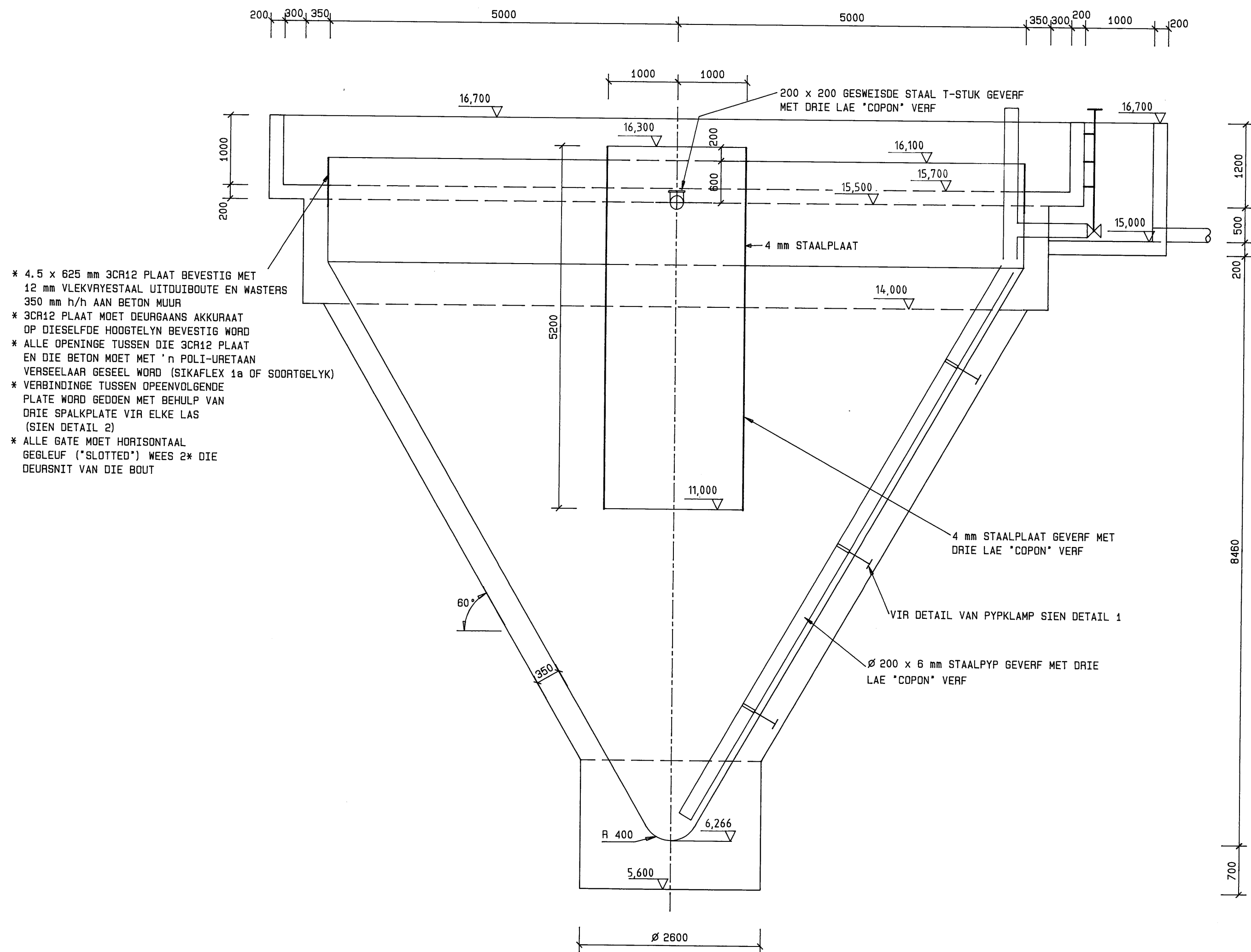
SNIT AA
