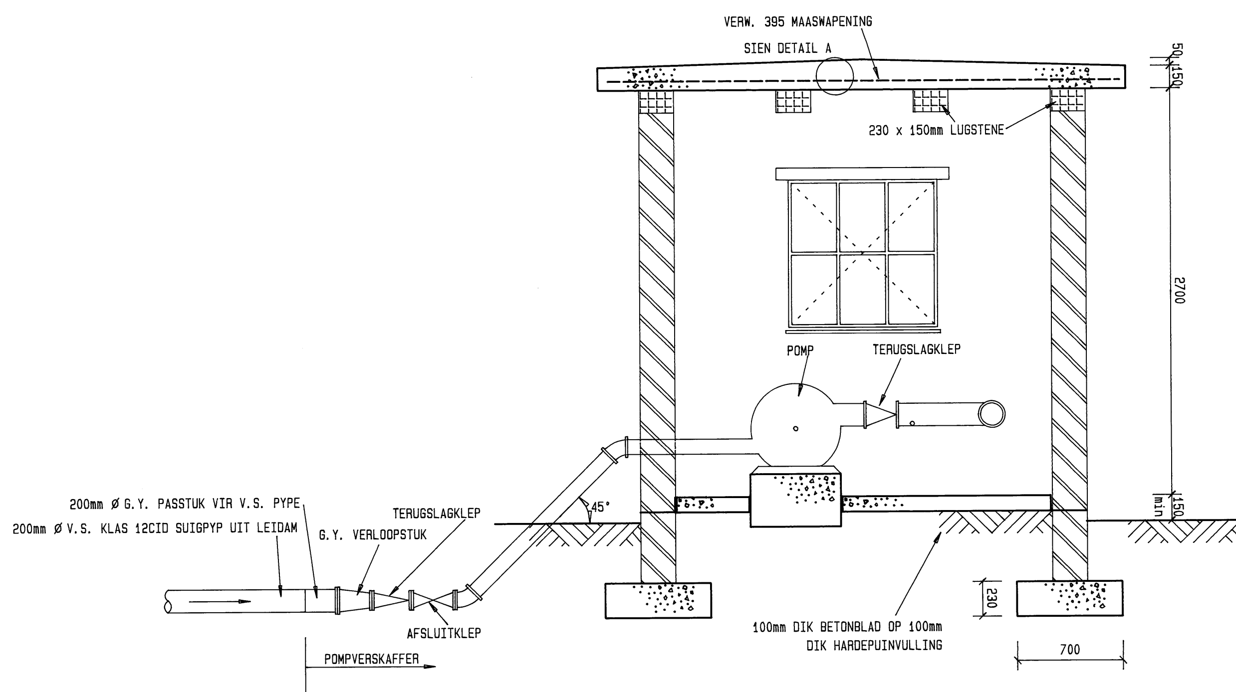
SNIT B - B
