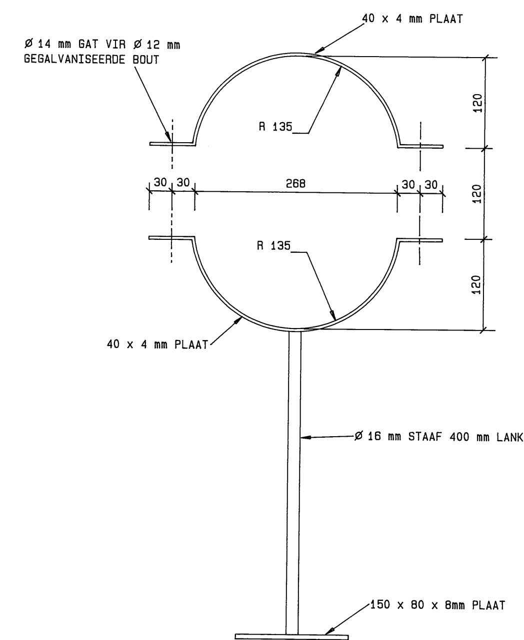
DETAIL 1
